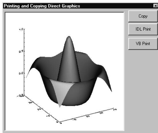
Figure 7-6: VBCopyPrint example
