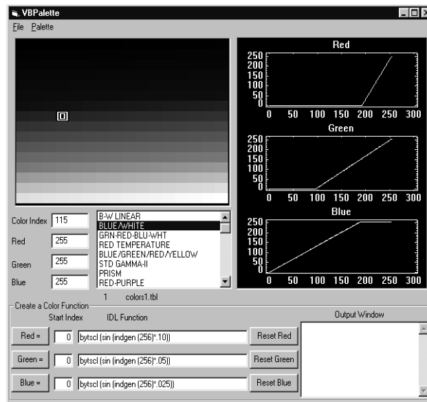
Figure 7-8: VBPalette Example
