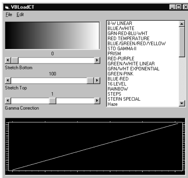
Figure 7-7: VBLoadCT Example
