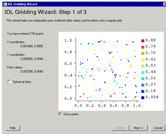
Figure 2-6: The IDL Gridding Wizard Step 1 of 3
