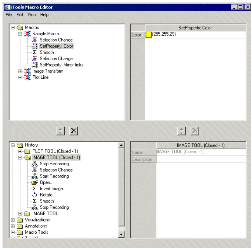
Figure 8-8: The Macro Editor
