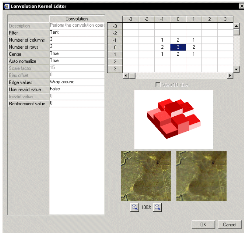
Figure 7-9: Convolution Kernel Editor
