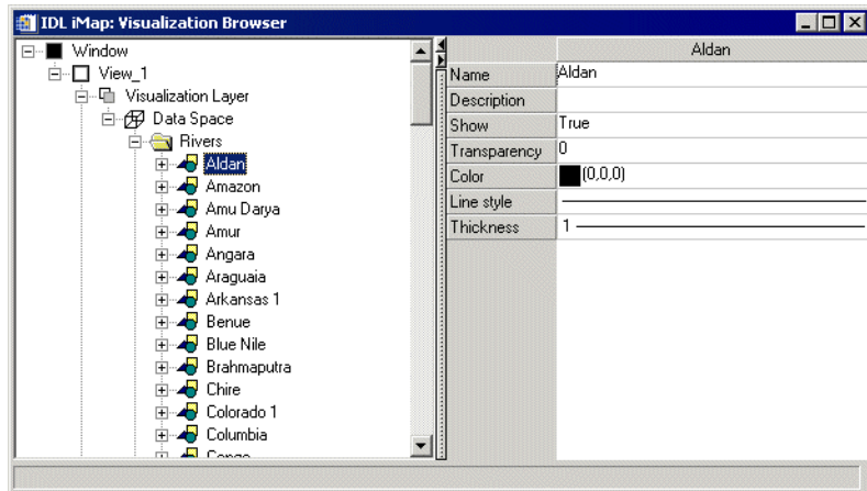
Figure D-30: Visualization Browser with ShapePolyline Properties Displayed
