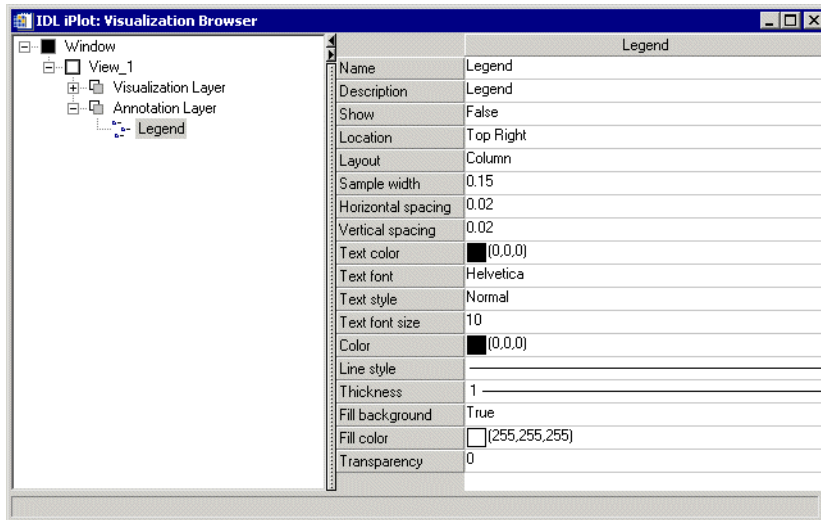
Figure D-32: Visualization Browser with Legend Properties Displayed
