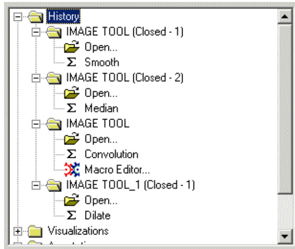
Figure 8-17: A History Example with Open and Closed Tools
