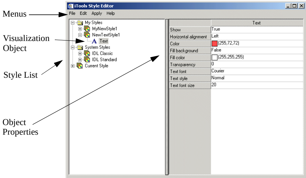
Figure 9-9: The iTools Style Editor
