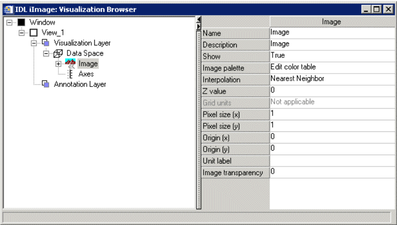
Figure D-11: Visualization Browser with Image Properties Displayed
