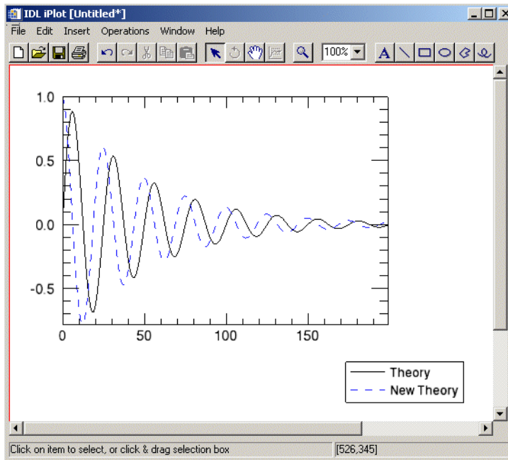
Figure 13-7: Plot and Overplot in iPlot with Legend Added for Each
