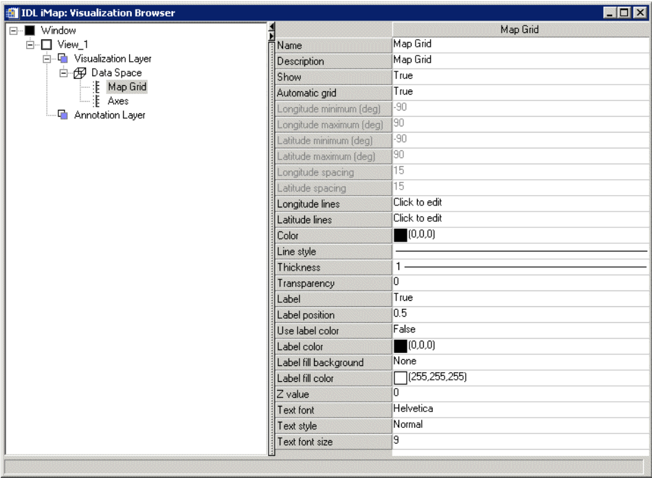
Figure D-28: Visualization Browser with Map Grid Object Properties Displayed
