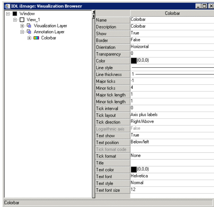
Figure D-22: Visualization Browser with Colorbar Properties Displayed
