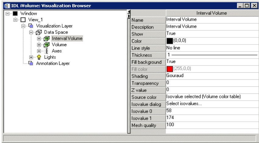
Figure D-20: Visualization Browser with Interval Volume Properties Displayed
