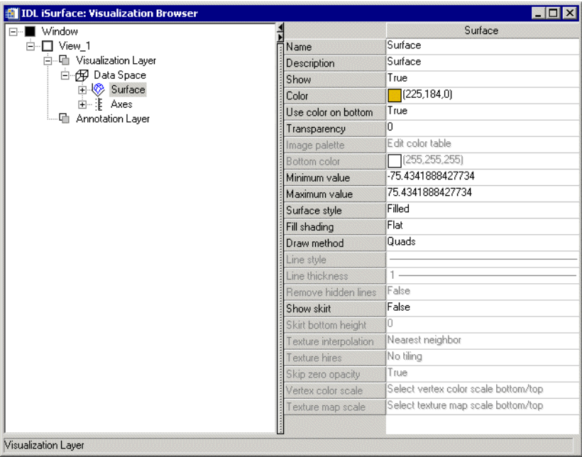
Figure D-14: Visualization Browser with Surface Properties Displayed
