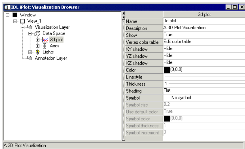
Figure D-13: Visualization Browser with 3D Plot Properties Displayed
