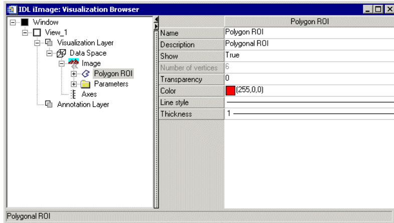
Figure D-26: Visualization Browser with Polygon ROI Properties Displayed
