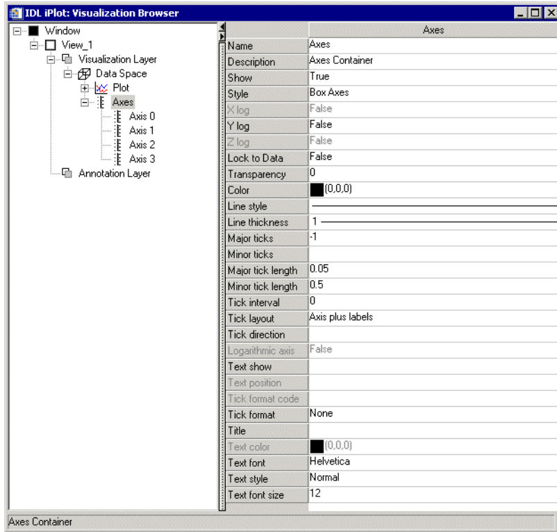
Figure D-24: Visualization Browser with Axis Properties Displayed
