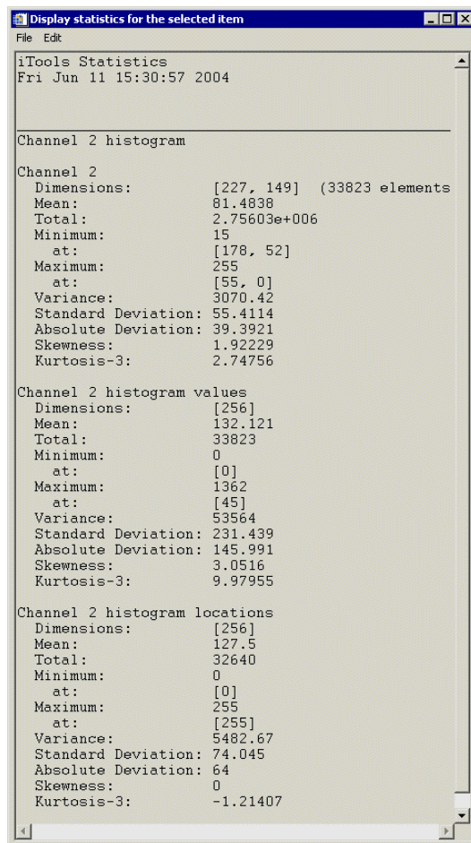
Figure 7-12: The iTools Statistics Window
