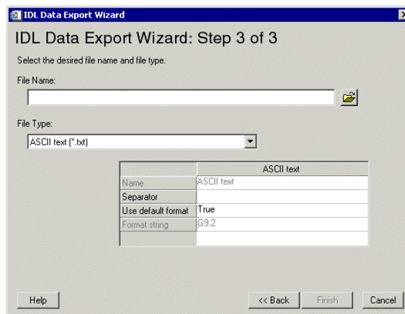
Figure 2-14: The IDL Data Export Wizard, Showing Step 3 of 3
