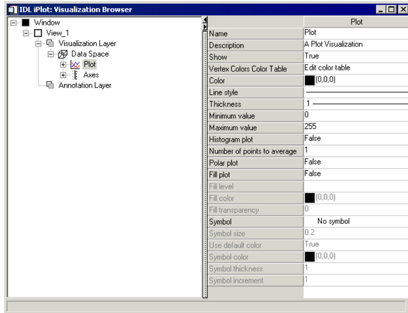
Figure D-12: Visualization Browser with Plot Properties Displayed
