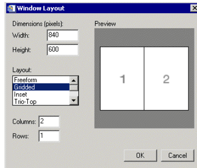
Figure 4-8: Window Layout Tool
